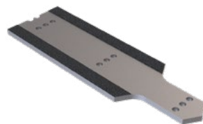
JK-740MAXCT PLOW BLADE, 3 HOLE, CONCRETE Fits: Kershaw and Knox Kershaw OEM part numbers: 116656, 194485, 9001087
