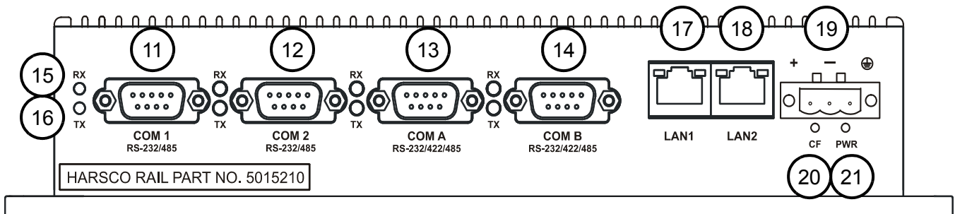
FIGURE 3 G5 JAM BOX
