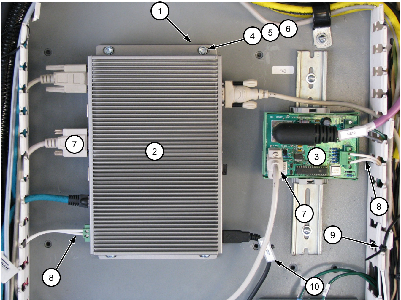
FIGURE 1 JUPITER G5 JAM BOX AND J42 CIRCUIT BOARD
