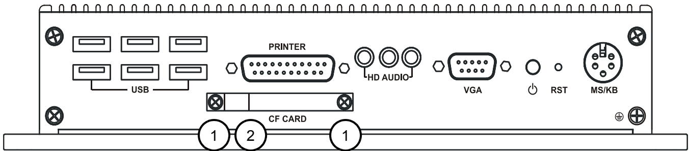
FIGURE 4 G5 JAM BOX
