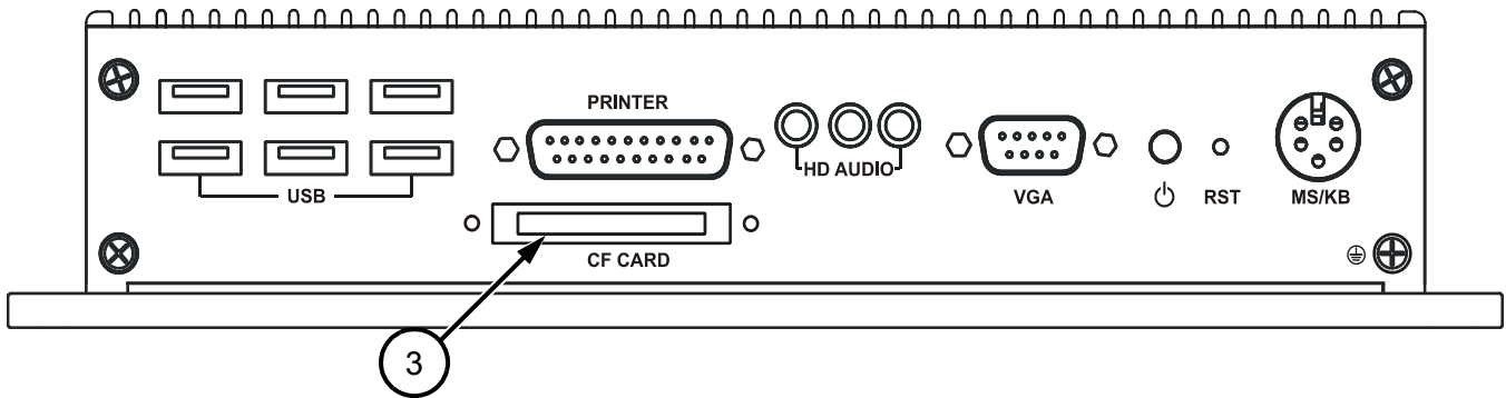
FIGURE 5 G5 JAM BOX
