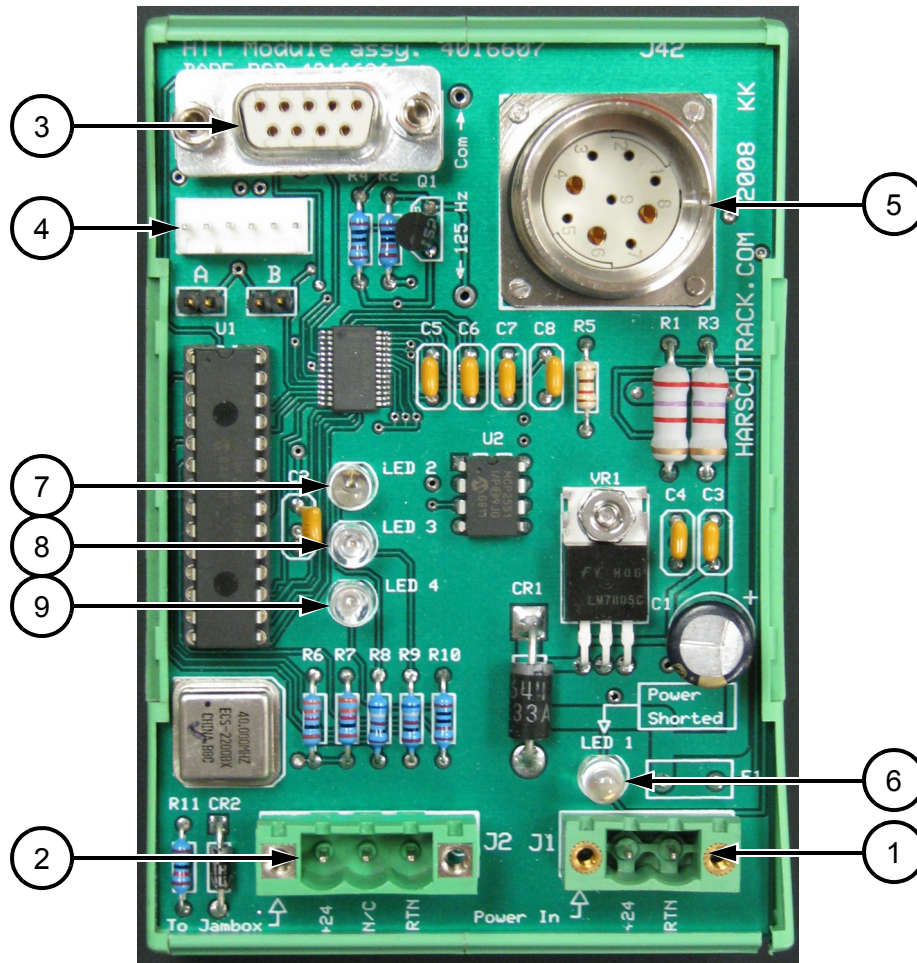
FIGURE 7 J42 BOARD
