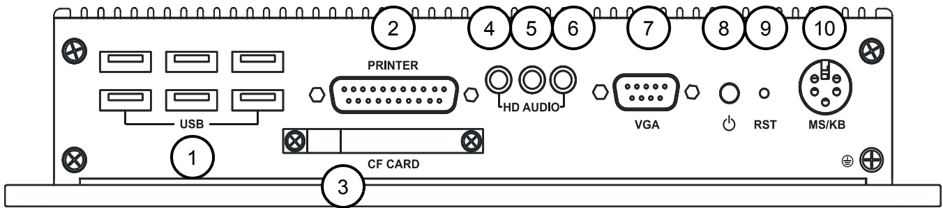
FIGURE 2 G5 JAM BOX
