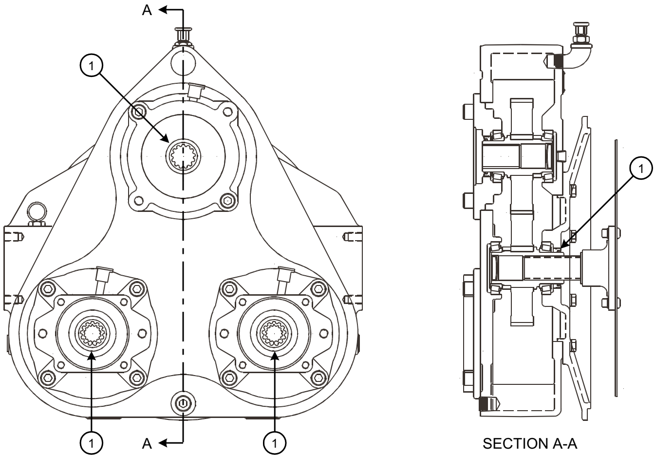
FIGURE 1 PUMP DRIVE SHAFT SEALS
