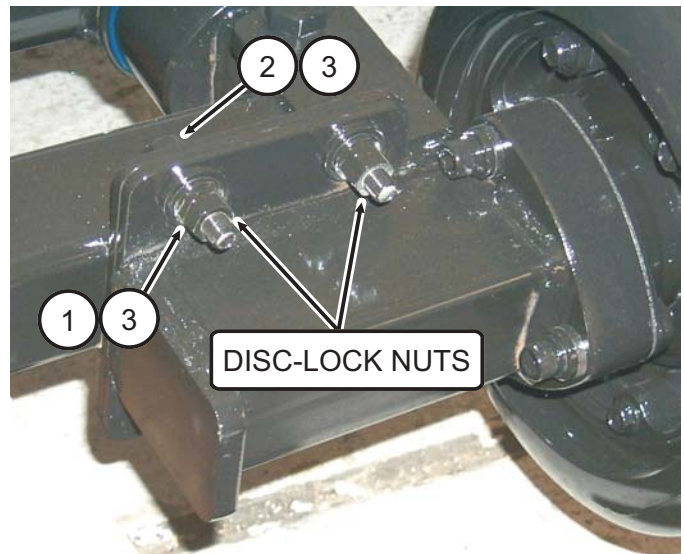
FIGURE 2 DISC-LOCK NUT LOCATION
